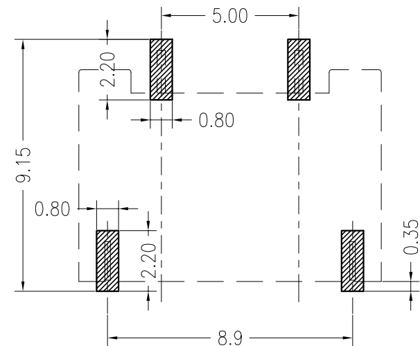
Board Layout
